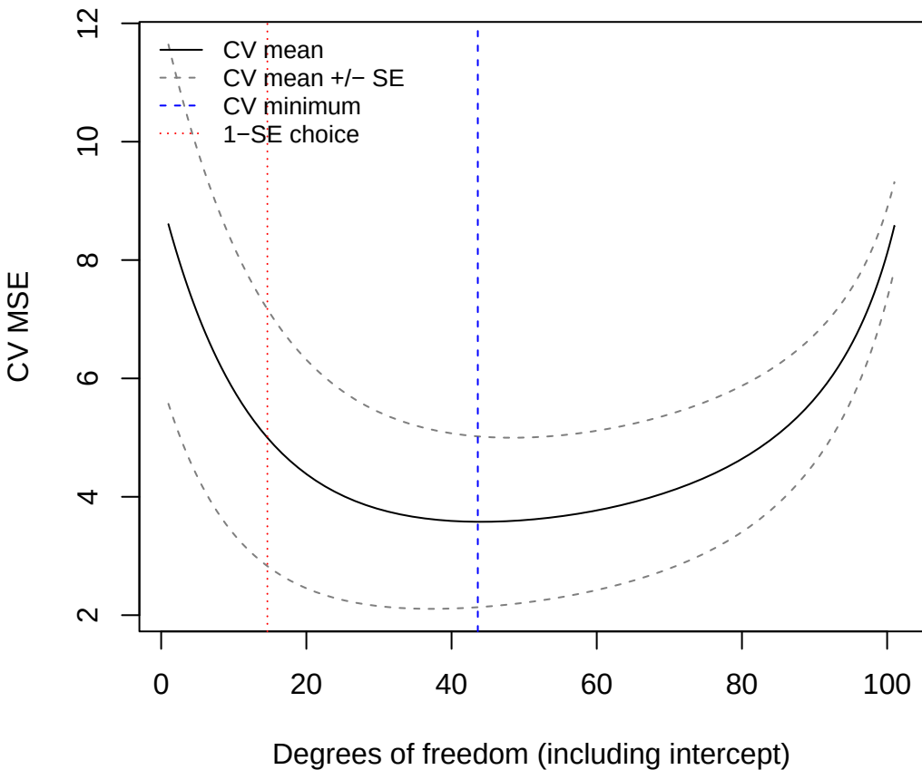
5 fold CV with one-SE bands
